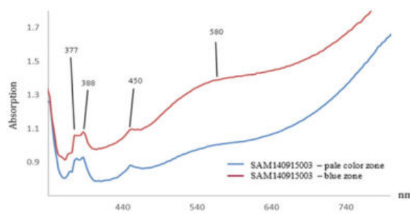
Figure 11. Non-polarized UV-Vis absorption spectra illustrating the differences in the blue and paler color zones of the mid 2014 slab sample no. SAM140915003, the spectra merely displayed up to 800 nm due to signal error at higher nm region.
