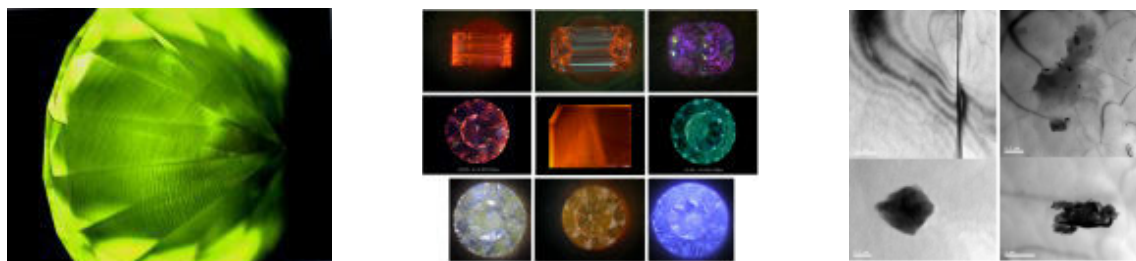
Figure 8. DiamondView: Shell-like curved lines provide evidence of CVD origin.
