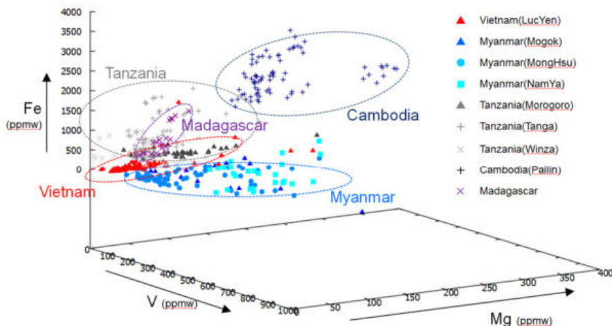
Figure 1. The 3D plot graph in Mg-V-Fe of rubies in this study.
