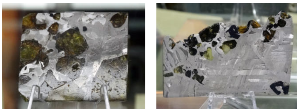
Figure 1. Pallasite slices of Fukang (left) and Seymchan (right).
