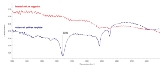
Figure 6. FTIR Spectra of unheated (blue trace) – and heated (red trace) yellow Sapphire.
