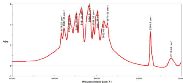
Figure 9. FTIR spectrum of Neriya star ruby shows \text{TiO}_2 contamination.
