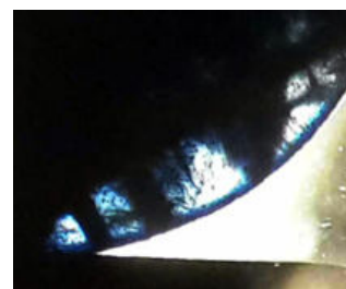
Figure 7. Color concentration along healed fissures and blue color rim along the mid 2014 stone surface outline seen under immersion in di-iodomethane solution. Photos: S. Saengbuangamlam.
