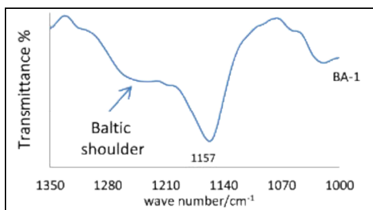
Figure 1. "Baltic shoulder" between 1250 \text{cm}^{-1} and 1175 \text{cm}^{-1} in Baltic amber sample spectrum.
