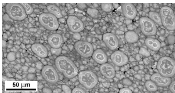
Figure 3. Backscattered electrons image (scanning electron microscope) of synthetic turquoise, showing a multitude of oolitic grains several ten micrometers in size.
