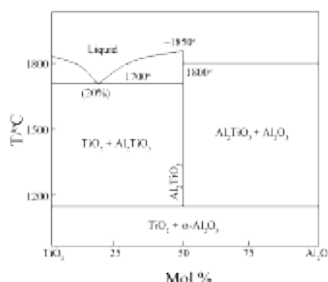
Figure 10. Phase diagram of \text{TiO}_2\text{:Al}_2\text{O}_3 after Goldberg (1968) in Abali (2011).
